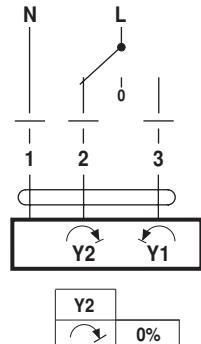
AC 230 V, 3-point
