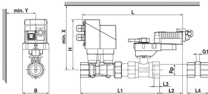
Dimensional drawings
