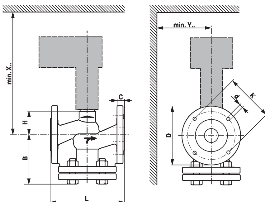
Dimensional drawings
