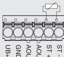
0...5/10 V + ST
