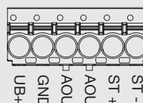
2 x 0...5/10 V
