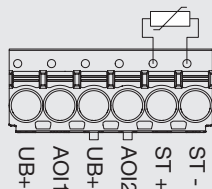
4...20 mA + ST
