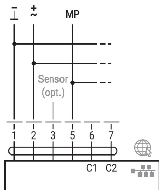
M-Bus with converter in parallel mode with BACnet/IP / Modbus TCP
