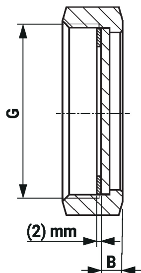
Dimensional drawings
