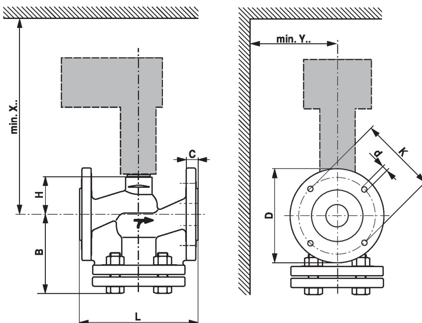
Dimensional drawings
