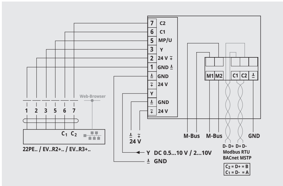
G-22PEM-A01 / M-Bus / 22PE.. / EV..R2+.. / EV..R3+.. / Modbus RTU / BACnet MSTP
