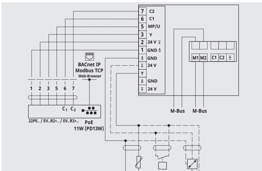
G-22PEM-A01 / M-Bus / 22PE.. / EV..R2+.. / EV..R3+.. / Modbus TCP / BACnet IP / PoE
