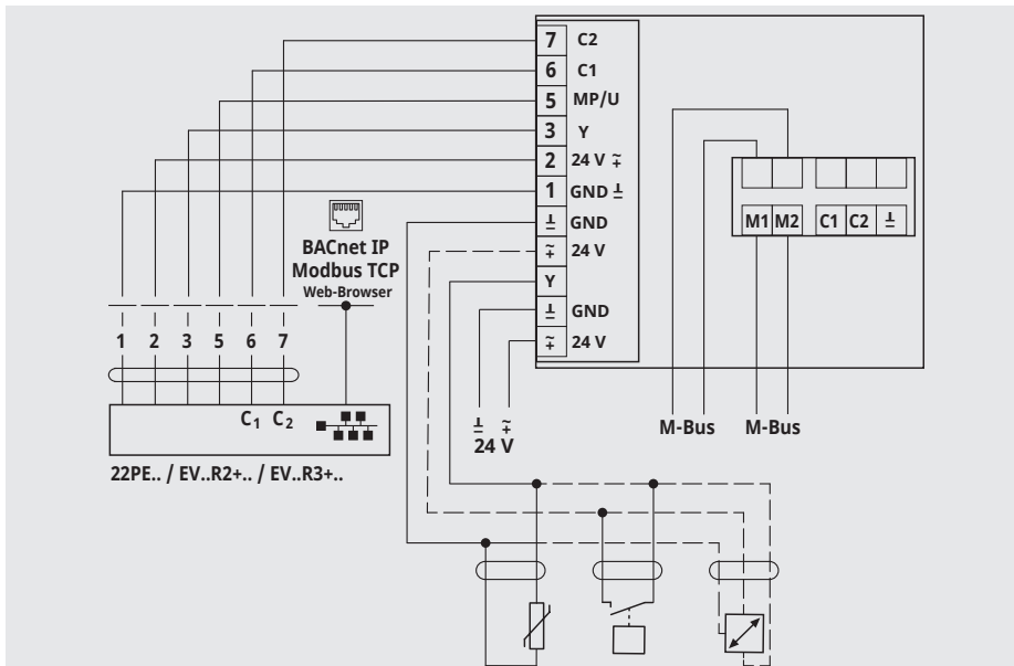
G-22PEM-A01 / M-Bus / 22PE.. / EV..R2+.. / EV..R3+.. / Modbus TCP / BACnet IP
