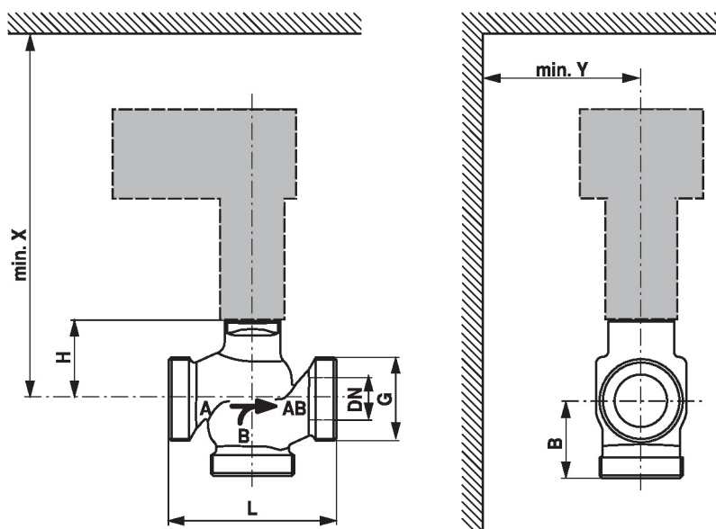
Dimensional drawings
