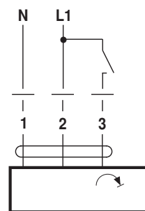
GR230A-R
