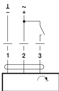
GR24A-R
