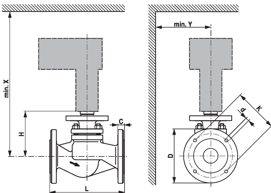
Dimensional drawings
