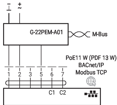
Connection with active sensor
